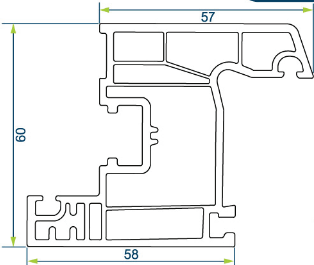
60 mm PENCERE KANAT PROFİLİ 60 mm WINDOW SASH PROFILE
