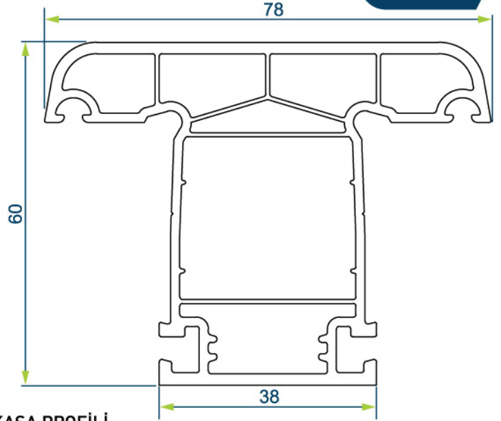
60 mm PERVAZLI KASA PROFİLİ 60 mm WIDE FRAME WITH BORDER
