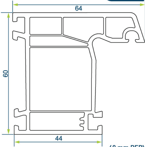
60 mm PERVAZLI KASA PROFİLİ 60 mm WIDE FRAME WITH BORDER
