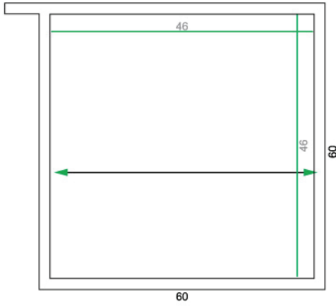
HAREKETLİ ORTA KAYIT MOVABLE MULLION PROFILE
