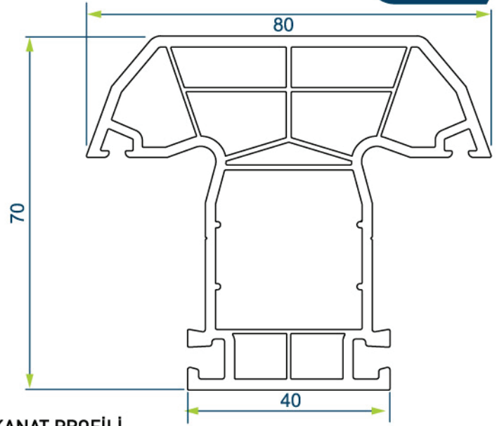
60 mm PENCERE KANAT PROFİLİ 60 mm WIDE FRAME WITH BORDER
