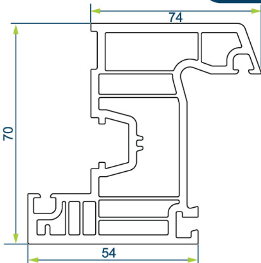
70 mm PENCERE KANAT PROFİLİ 70 mm WINDOW SASH PROFILE
