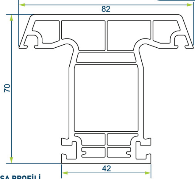
70 mm PERVAZLI KASA PROFİLİ 70 mm WIDE FRAME WITH BORDER
