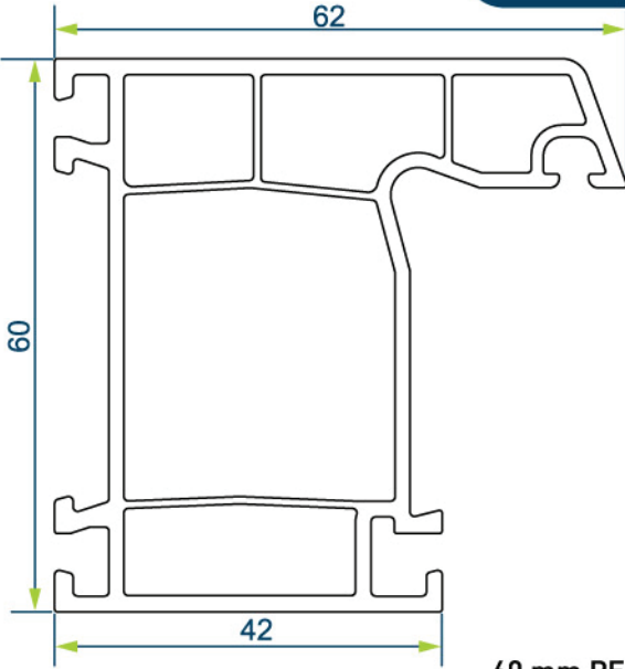
60 mm PERVAZLI KASA PROFİLİ 60 mm WIDE FRAME WITH BORDER
