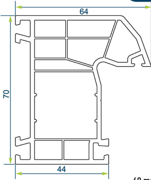
70 mm KASA PROFİLİ 70 mm FRAME PROFILE
