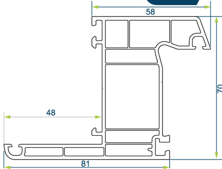
70 mm PENCERE KANAT PROFİLİ 70 mm WINDOW SASH PROFILE
