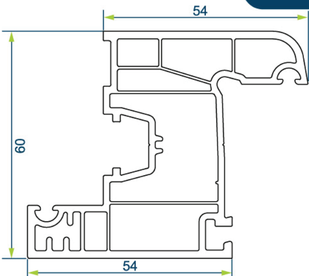
60 mm PENCERE KANAT PROFİLİ 60 mm WINDOW SASH PROFILE
